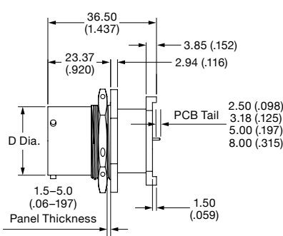
Double Flange
