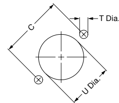
Flange Mounting
